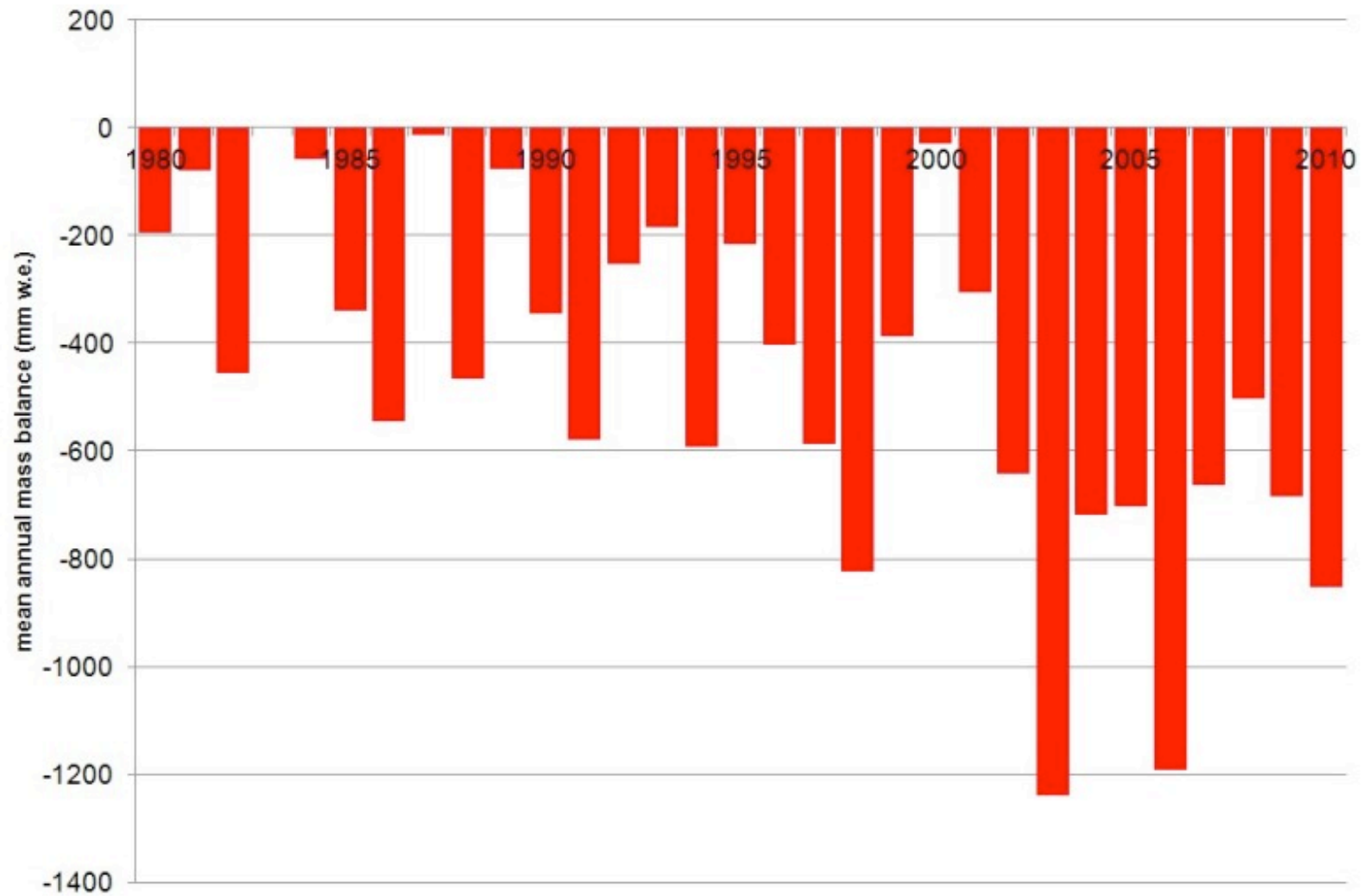
Figure 1: Mean annual mass balance of reference glaciers. pdf
