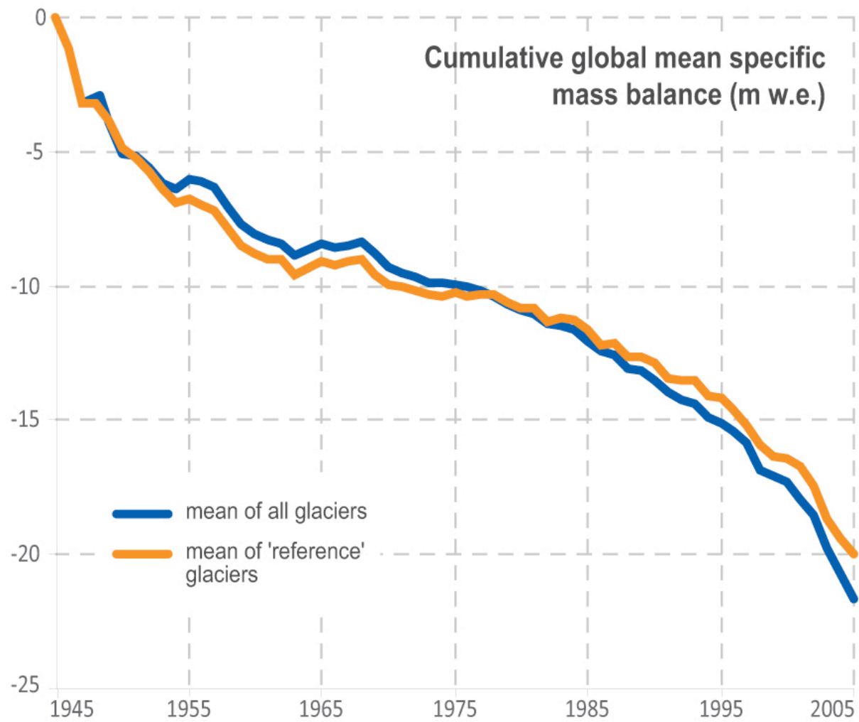
Fig. 5.9 Cumulative specific mass balance
